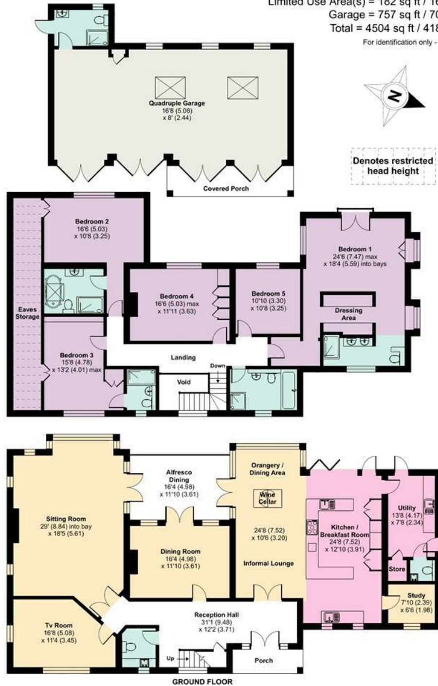
GROUND FLOOR
